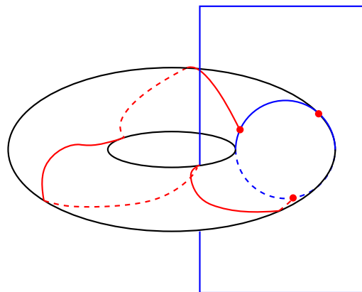
Fig. 4.8 The Poincaré section of a torus is a circle. The dynamics on the torus becomes a mapping of the circle onto itself.
