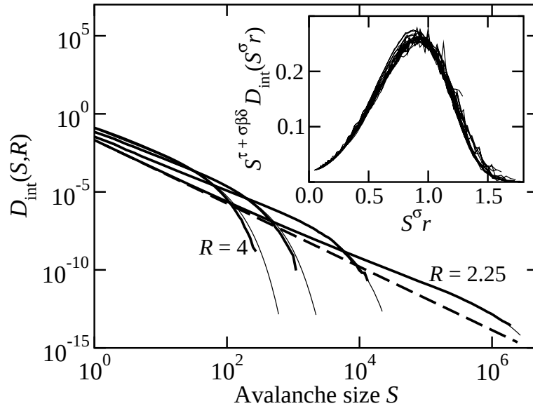
Fig. 12.13 Avalanche size distribution. The distribution of avalanche sizes in our model for hysteresis. Notice the logarithmic scales. (We can measure a D(S) value of 10^{-14} by running billions of spins and binning over ranges \Delta S \sim 10^5 .) (i) Although only at R_c \approx 2.16 do we get a pure power law (dashed line, D(S) \propto S^{-\bar{\tau}} ), we have large avalanches with hundreds of spins even a factor of two away from the critical point. (ii) The curves have the wrong slope except very close to the critical point; be warned that a power law over two decades (although often publishable [84]) may not yield a reliable exponent. (iii) The scaling curves (thin lines) work well even far from R_c . Inset: We plot D(S)/S^{-\bar{\tau}} versus S^\sigma(R - R_c)/R to extract the universal scaling curve \mathcal{D}(X) (eqn 12.14). Varying the critical exponents and R_c to get a good collapse allows us to measure the exponents far from R_c , where power-law fits are still unreliable (Exercise 12.12(g)).
