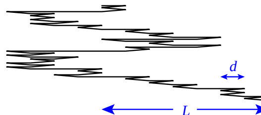
Fig. 5.19 Rubber band. Simple model of a rubber band with N = 100 segments. The beginning of the polymer is at the top; the end is at the bottom; the vertical displacements are added for visualization.
