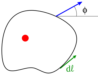
Fig. 9.21 Looping the defect. The curve D encircles the defect once; d\ell is a unit vector tangent to D running counter-clockwise. Define \phi to be the angle between the unit vector \mathbf{m} and the x -axis.
