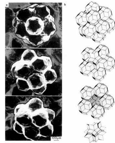
Fig. 9.1 Quasicrystals. Crystals are surely the oldest known of the broken-symmetry phases of matter. In the past few decades, we have uncovered an entirely new class of quasicrystals , here [72] with icosahedral symmetry. Note the five-fold structures, forbidden in our old categories.
