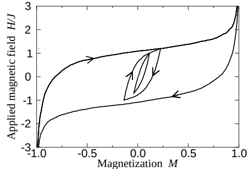
Fig. 8.15 Hysteresis loop with subloops for our model. As the external field is raised and lowered (vertical), the magnetization lags behind—this is called hysteresis . The magnetization curves here look macroscopically smooth.
