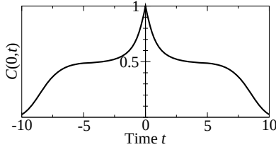
Fig. 10.10 Time-time correlation function. The time-time correlation function C(\mathbf{r} = \mathbf{0}, \tau) for the same hypothetical system whose susceptibility was shown in Fig. 10.9.
