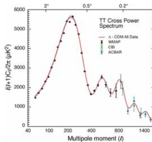
Fig. 10.14 Correlation function of microwave radiation in Fourier space, from the NASA/WMAP Science Team [137]. Temperature variations of the microwave background radiation, written in spherical harmonics (roughly an angular Fourier transform). You can think of l for the multipole moment as roughly corresponding to wavevector k_l = 2\pi l/L . 32 The curve through the data is a more complete theoretical fit, similar in spirit to this exercise.
