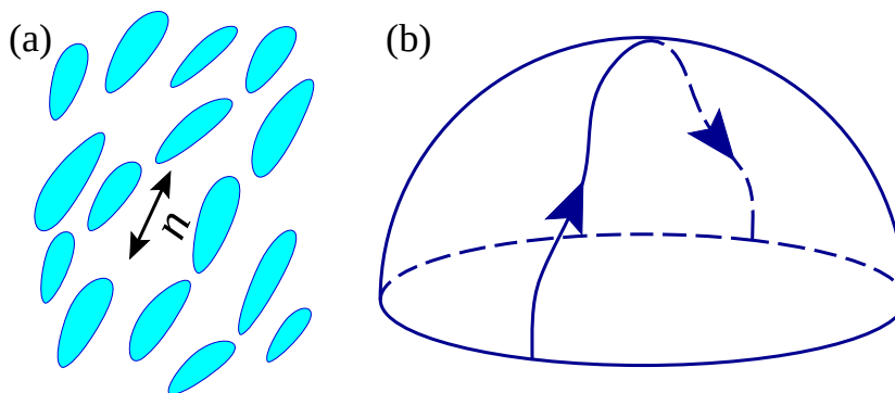
Fig. 9.5 Nematic order parameter space. (a) Nematics are made up of long, thin molecules that prefer to align with one another. (Liquid crystal watches are made of nematics.) Since they do not care much which end is up, their order parameter is not a vector \hat{n} along the axis of the molecules, but is instead a unit vector up to the equivalence \hat{n} \equiv -\hat{n} . (b) The nematic order parameter space is a half-sphere, with antipodal points on the equator identified. Thus, for example, the route shown over the top of the hemisphere is a closed path; the two intersections with the equator correspond to the same orientations of the nematic molecules in space.
