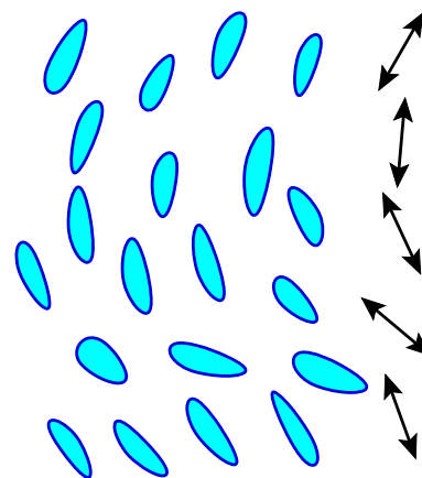
Fig. 9.10 Nematic liquid crystals: rotational waves. Nematic liquid crystals also have low-frequency rotational waves.
