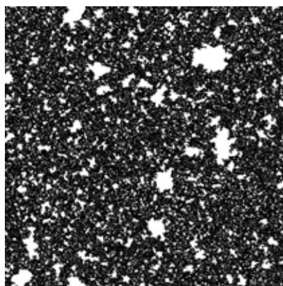
Fig. 12.2 Percolation transition. A percolation model on the computer, where bonds between grid points are removed rather than circular holes. Let the probability of removing a bond be 1 - p ; then for p near one (no holes) the conductivity is large, but decreases as p decreases. After enough holes are punched (at p_c = 1/2 for this model), the biggest cluster just barely hangs together, with holes on all length scales. At larger probabilities of retaining bonds p = 0.51 , the largest cluster is intact with only small holes (bottom left); at smaller p = 0.49 the sheet falls into small fragments (bottom right; shadings denote clusters). Percolation has a phase transition at p_c , separating a connected phase from a fragmented phase (Exercises 2.13 and 12.12).
