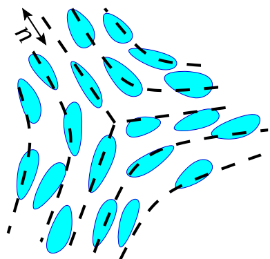
Fig. 9.14 Defect line in a nematic liquid crystal. You cannot lasso the sphere, but you can lasso a hemisphere! Here is the defect corresponding to the path shown in Fig. 9.5(b). As you pass clockwise around the defect line, the order parameter rotates counter-clockwise by 180^\circ . This path on Fig. 9.5(b) would actually have wrapped around the right-hand side of the hemisphere. Wrapping around the left-hand side would have produced a defect which rotated clockwise by 180^\circ . The path in Fig. 9.5(b) is half-way in between, and illustrates that these two defects are really not different topologically (Exercise 9.1).
